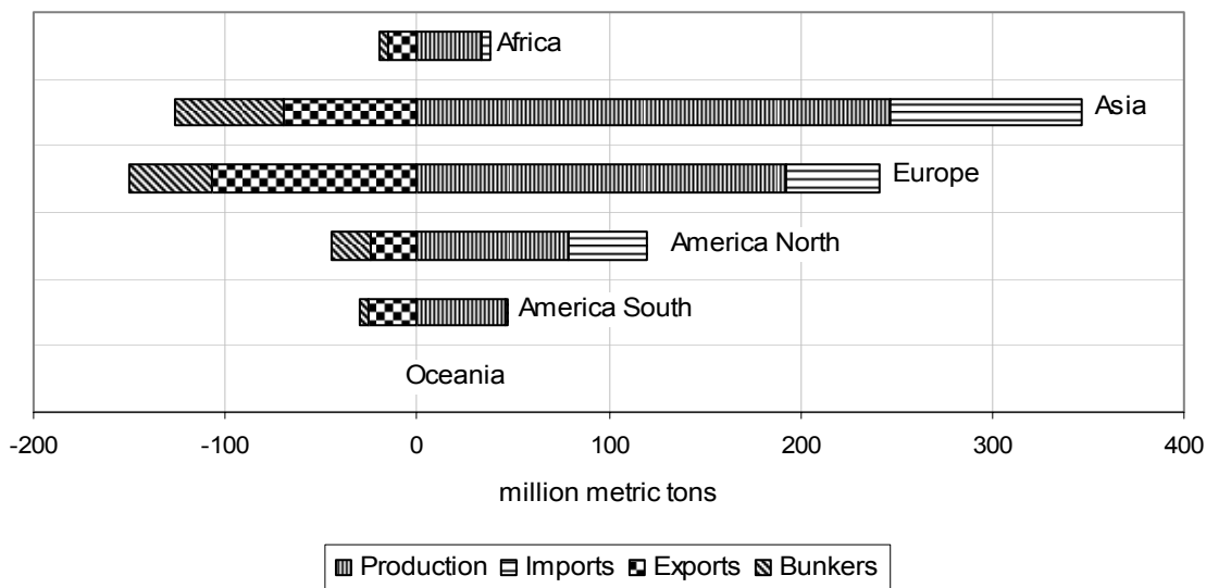
Production, trade and bunkers of residual fuel oil by region, 2004
