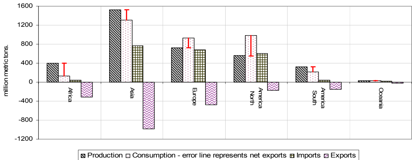
Production, trade and consumption of crude petroleum by region, 2004
