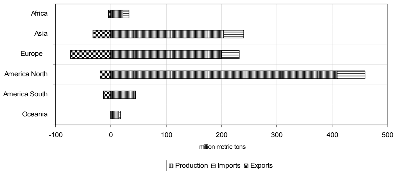
Production and trade of motor gasoline, by region, 2004
