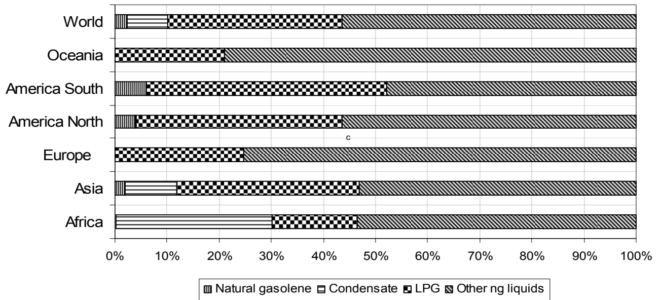
Production of natural gas liquids from plants by type, by region, 2004
