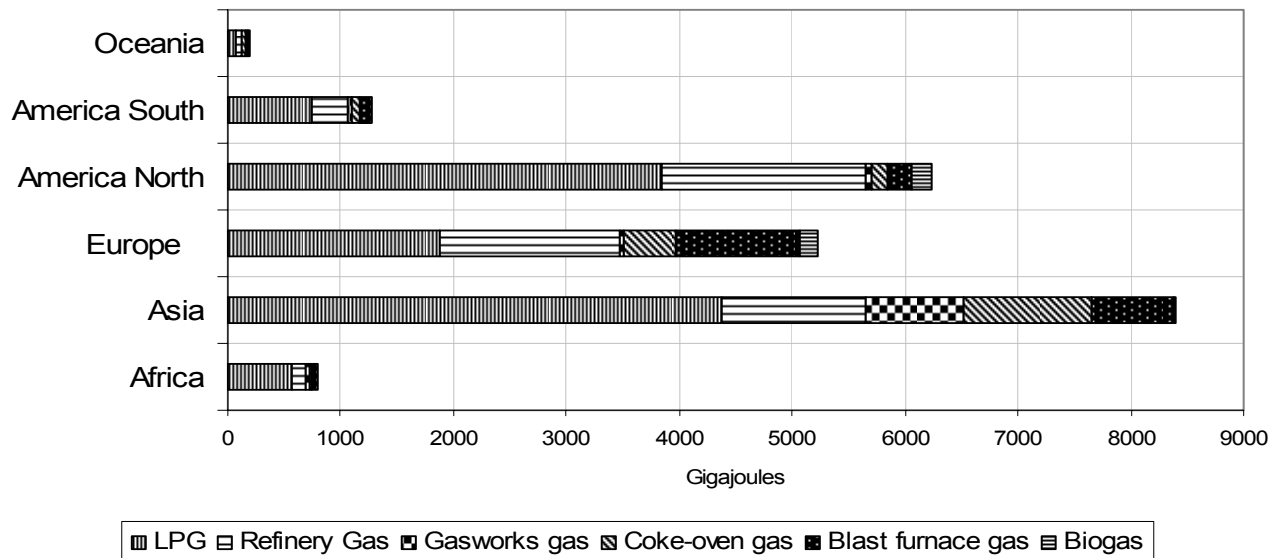
Production of other gases by region, by type, 2004
