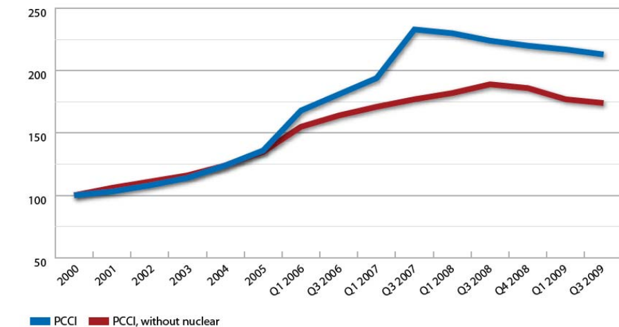
Figure 8 IHS CERA Power Capital Costs Index, 2000-2009
