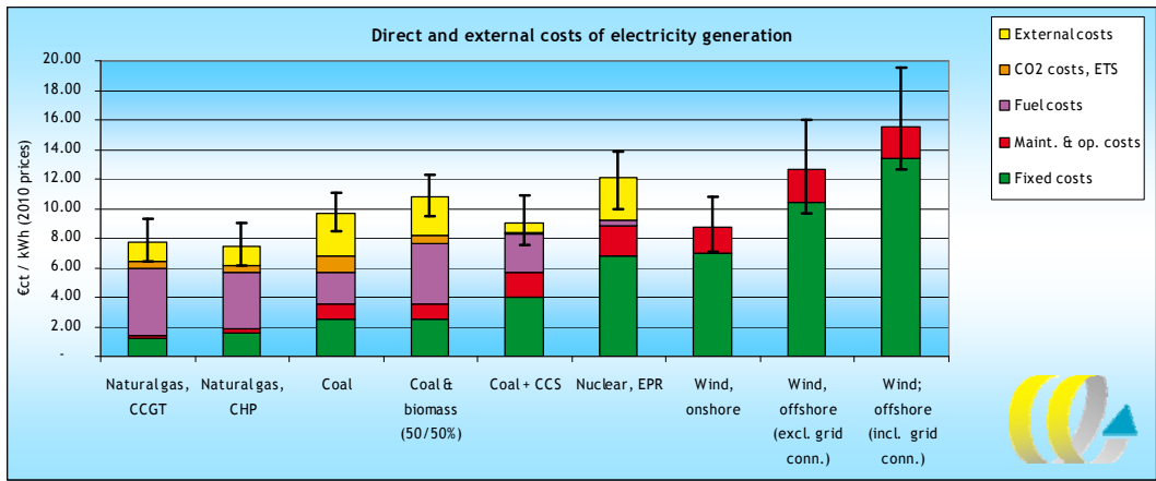
Figure 1 Costs of electricity generation including external costs
