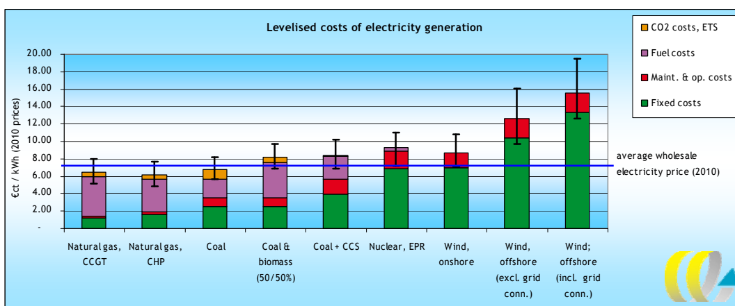
Figure 16 Direct costs of electricity generation, investor's perspective in 2011
