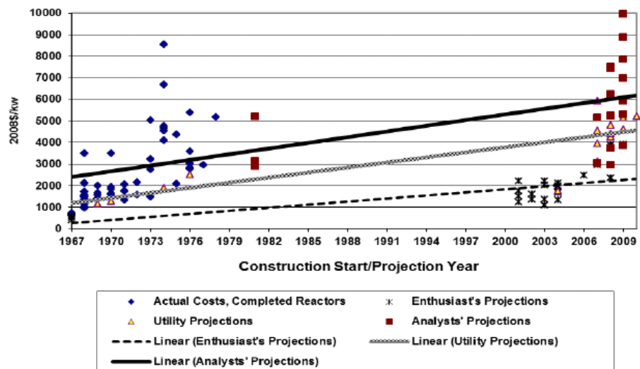
Figure 9 Construction cost estimates versus actual costs
