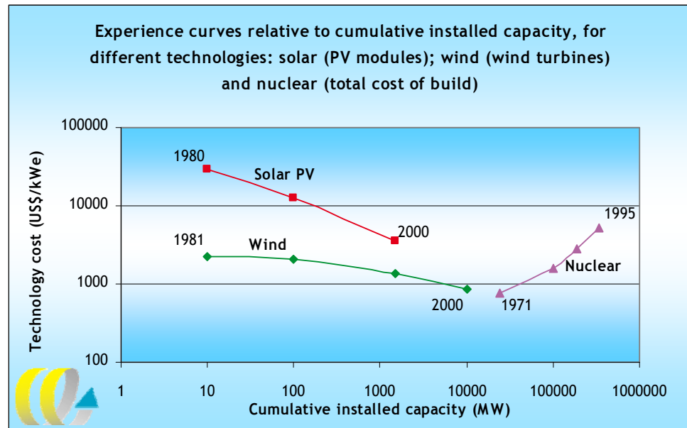
Figure 2 Experience curves for technology options. Cost relative to cumulative installed capacity of nuclear, wind and solar PV
