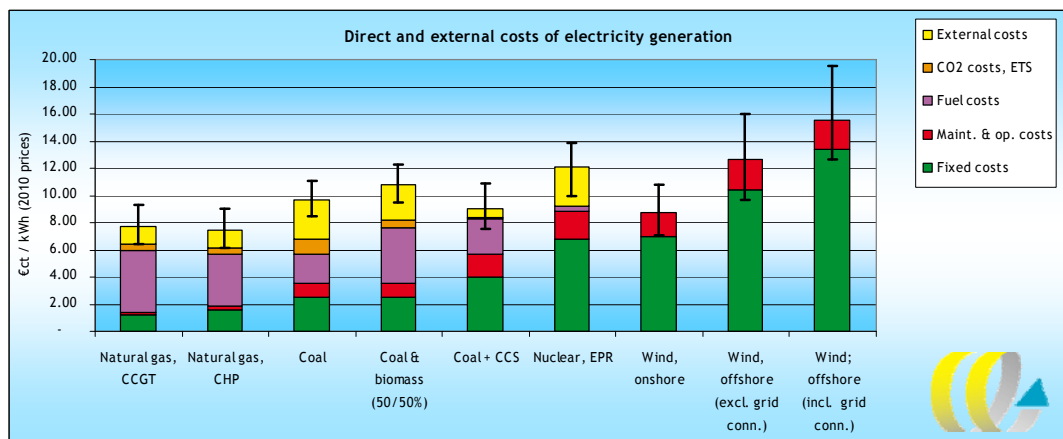
Figure 6 Costs of electricity generation including external costs
