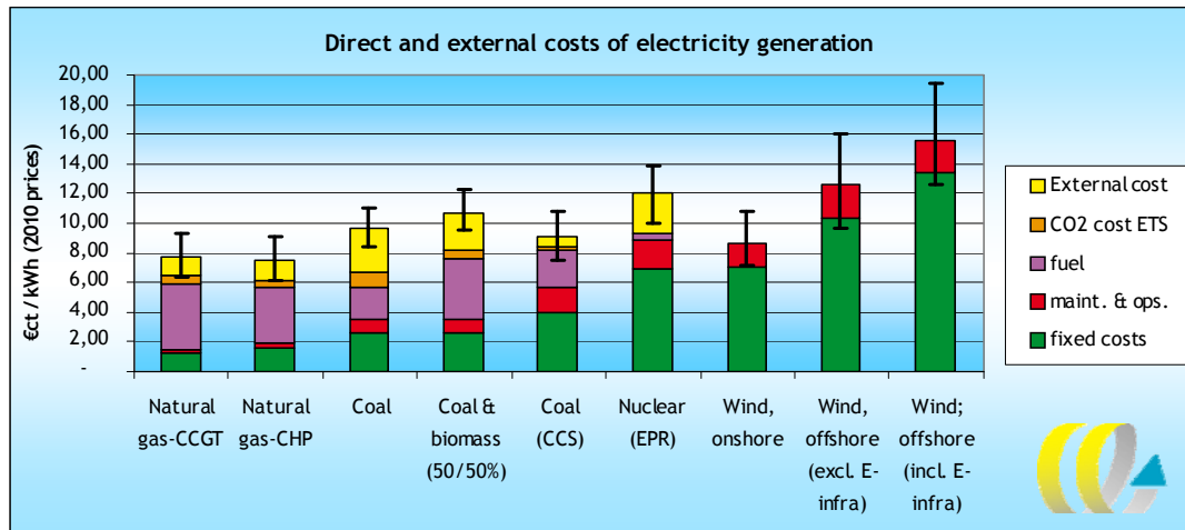
Figure 18 Costs of electricity generation including external costs of environmental damages, uninsured damage costs of accidents, and land use changes
