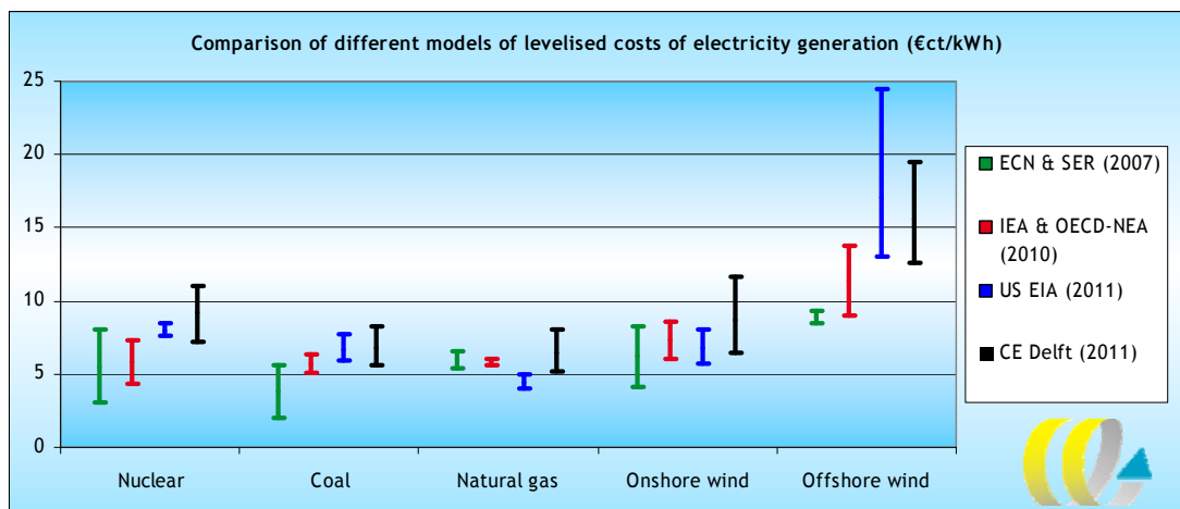
Figure 17 Comparison of different models of levelised costs of electricity generation
