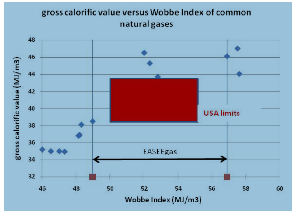
Figure 15 Comparison of gas quality range for Europe (EASEE) and for USA
