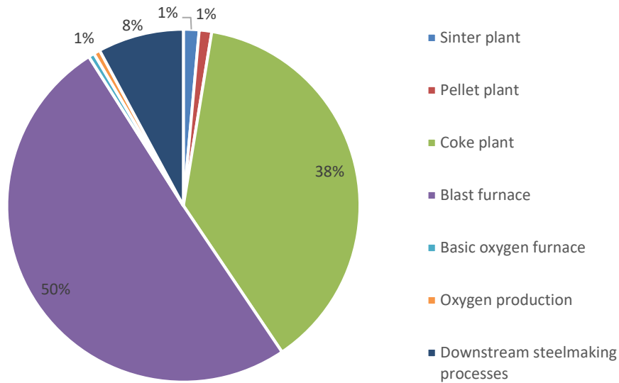
Figure 6. Total energy consumption distribution in steelmaking process
