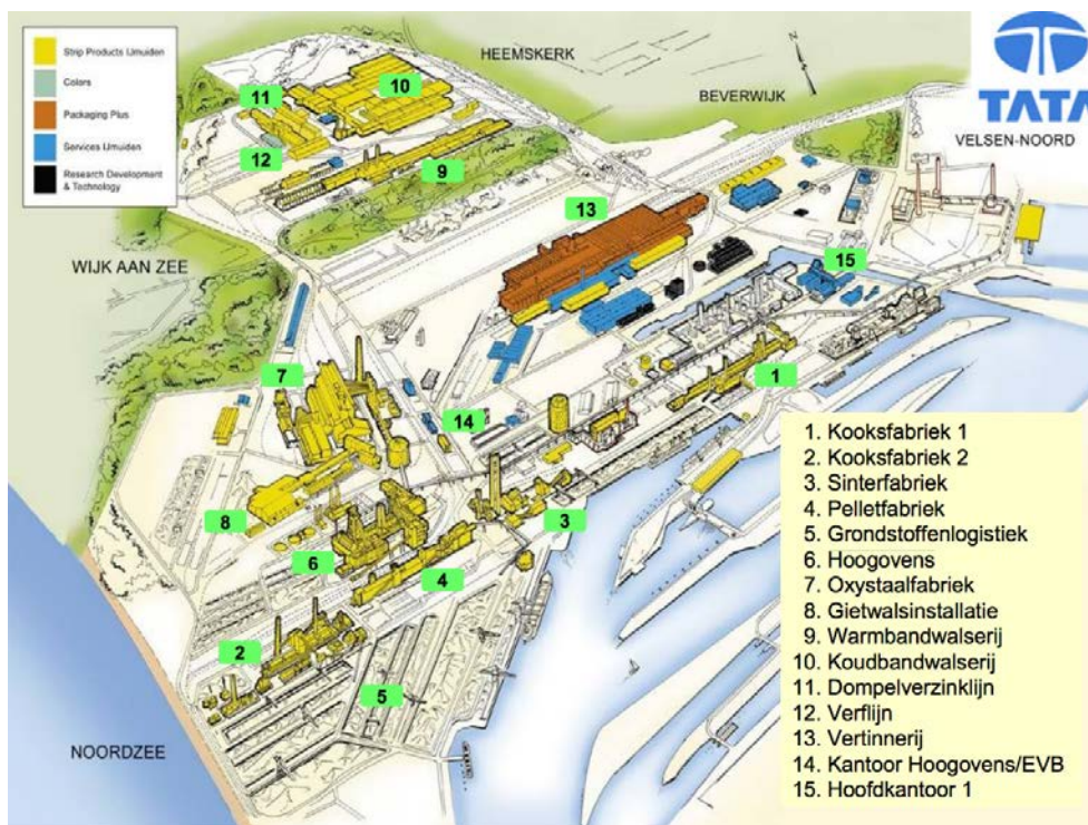
Figure 2. Site layout overview at Tata Steel IJmuiden (Tata Steel Europe, 2016)
