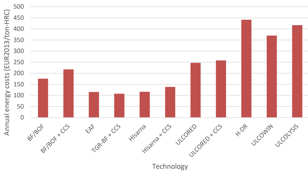
Figure 38. Annual energy costs for steelmaking options based on a 2050 low energy cost scenario in the Netherlands
