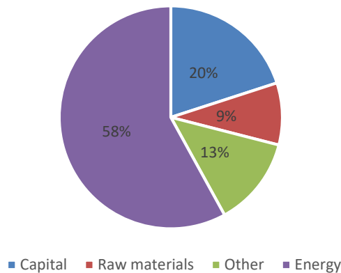
Figure 33. Cost breakdown for CO 2 capture (MEA solvent) at a conventional steel mill power plant
