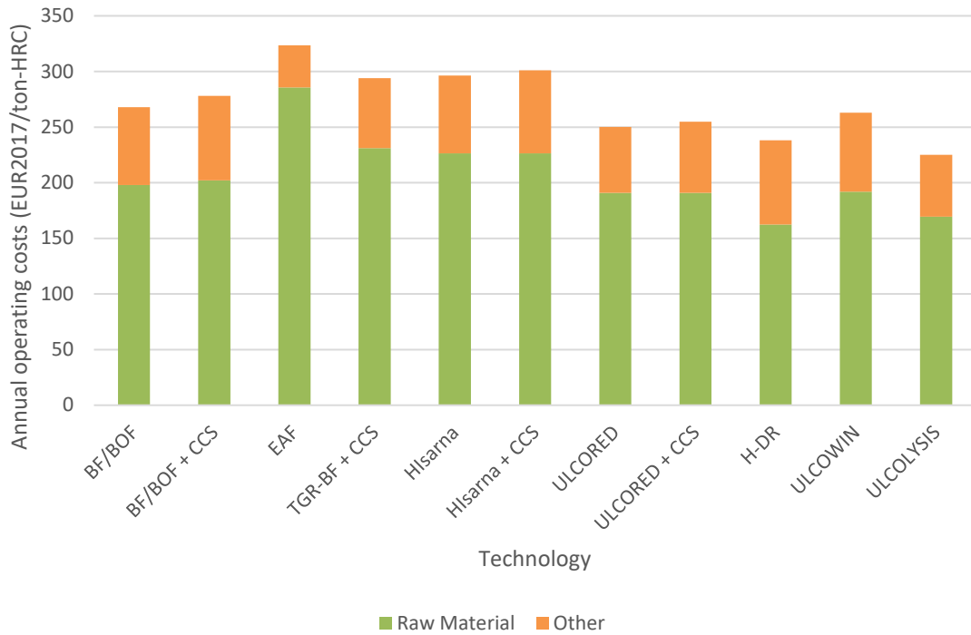
Figure 35. Annual operating costs of decarbonisation options (excluding energy)
