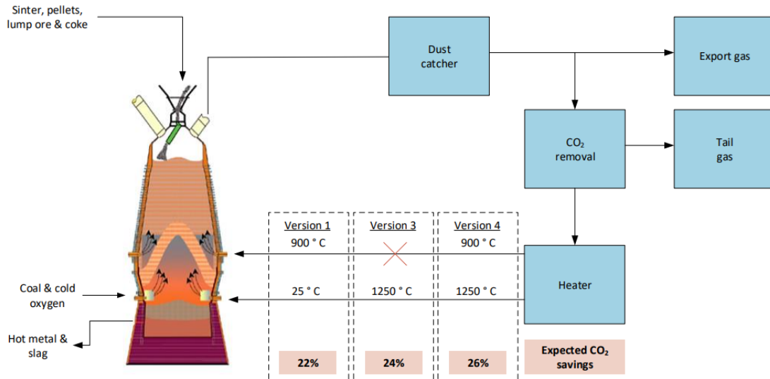
Figure 11. Simplified process flow diagram of considered variations of TGR-BF
