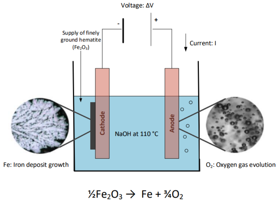
Figure 16. Basic schematic of iron ore electrolysis
