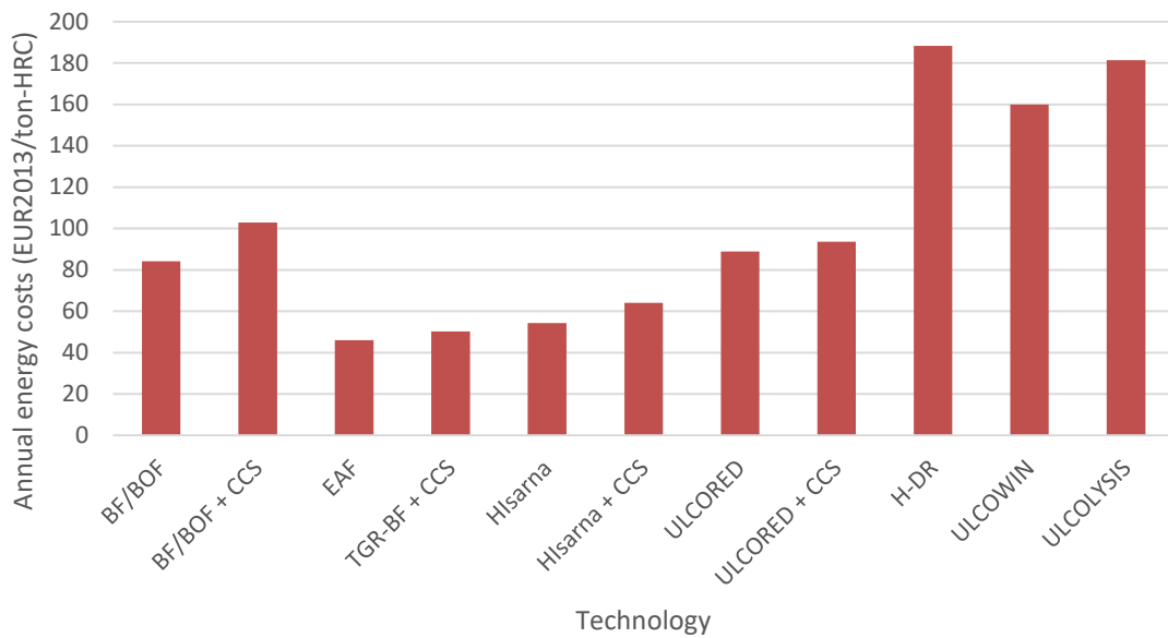
Figure 36. Annual energy costs for steelmaking options based on 2017 historical prices in the Netherlands
