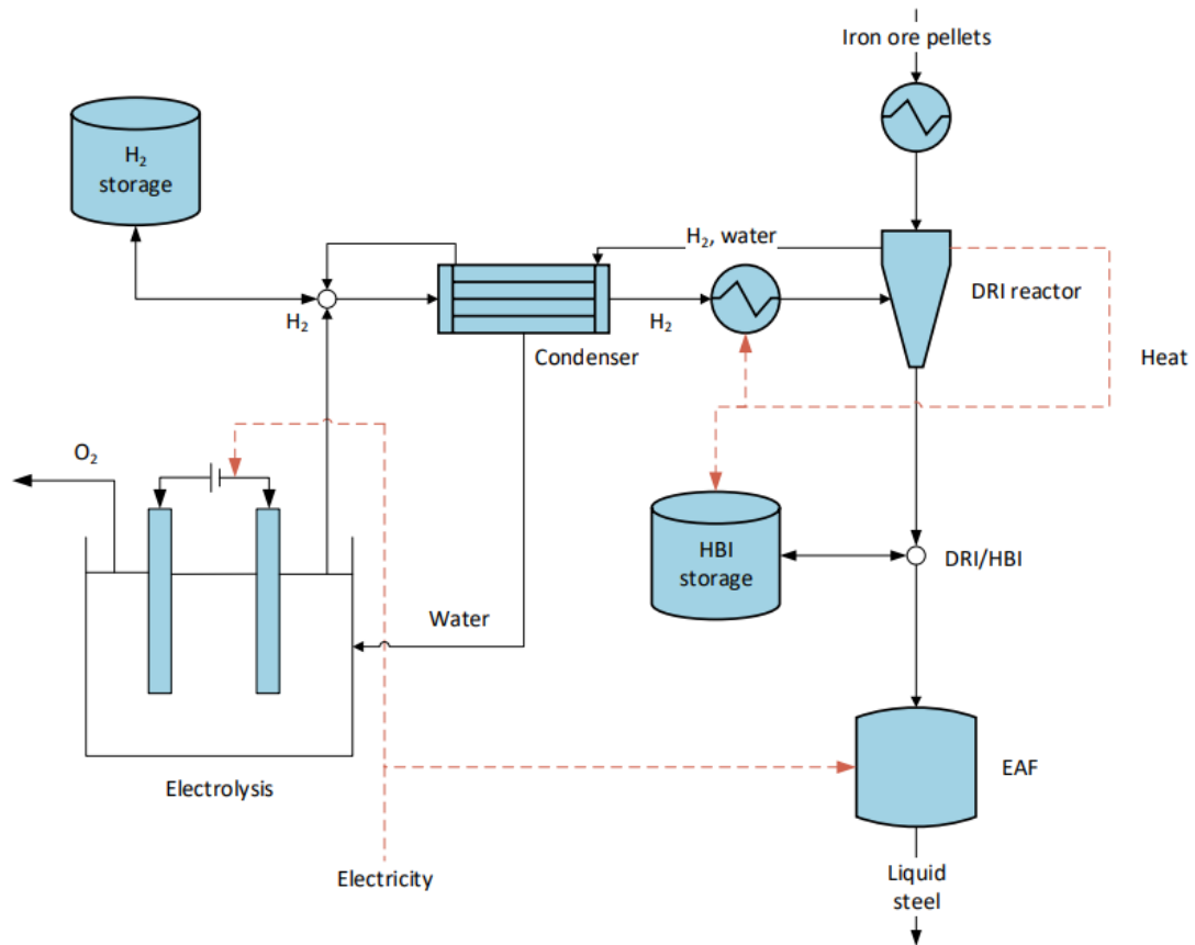
Figure 15. Example schematic of hydrogen-based direct reduction
