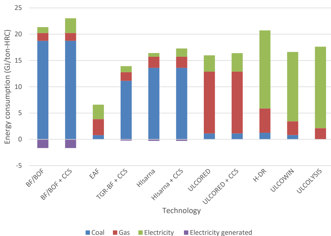
Figure 30. Annual energy consumption of decarbonisation options relative to the current BF/BOF process
