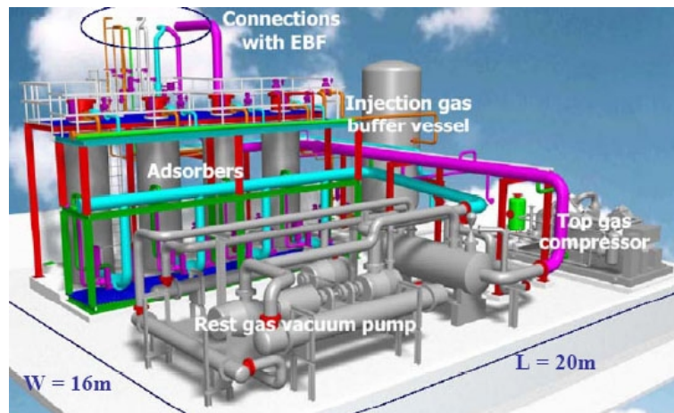
Figure 19. Plant layout of the VPSA implemented by Air Liquide in the ULCOS TGR-BF in Luleå.
