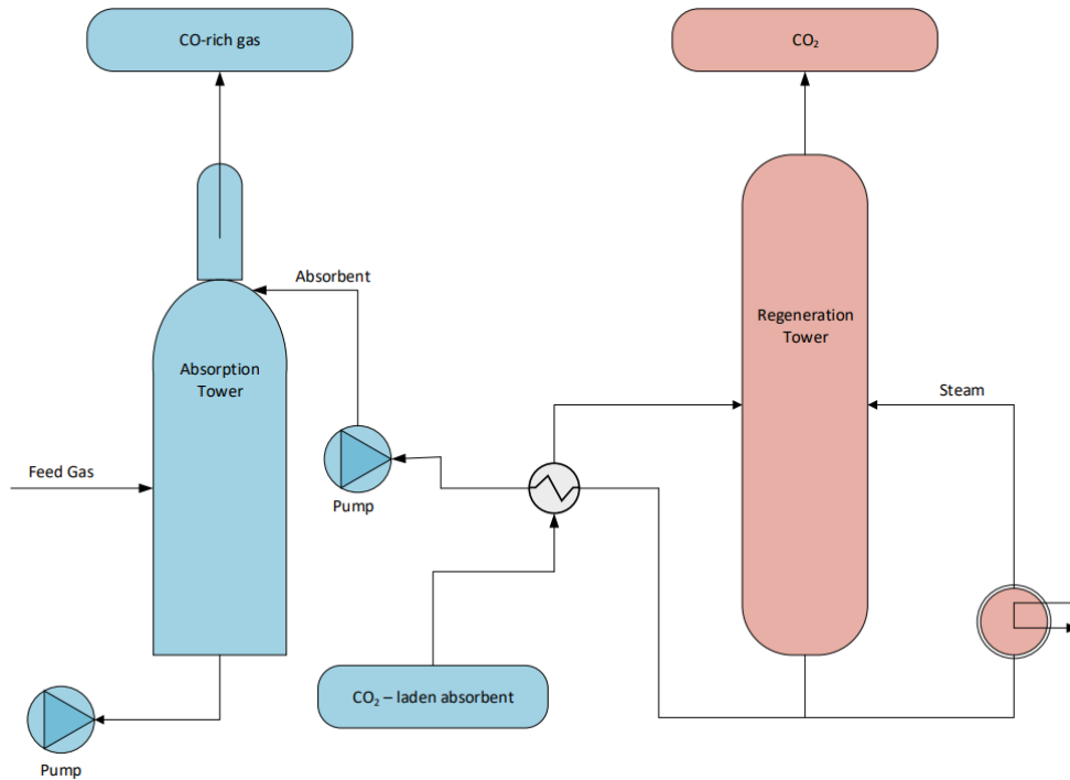
Figure 17. Schematic of chemical absorption-based CCS
