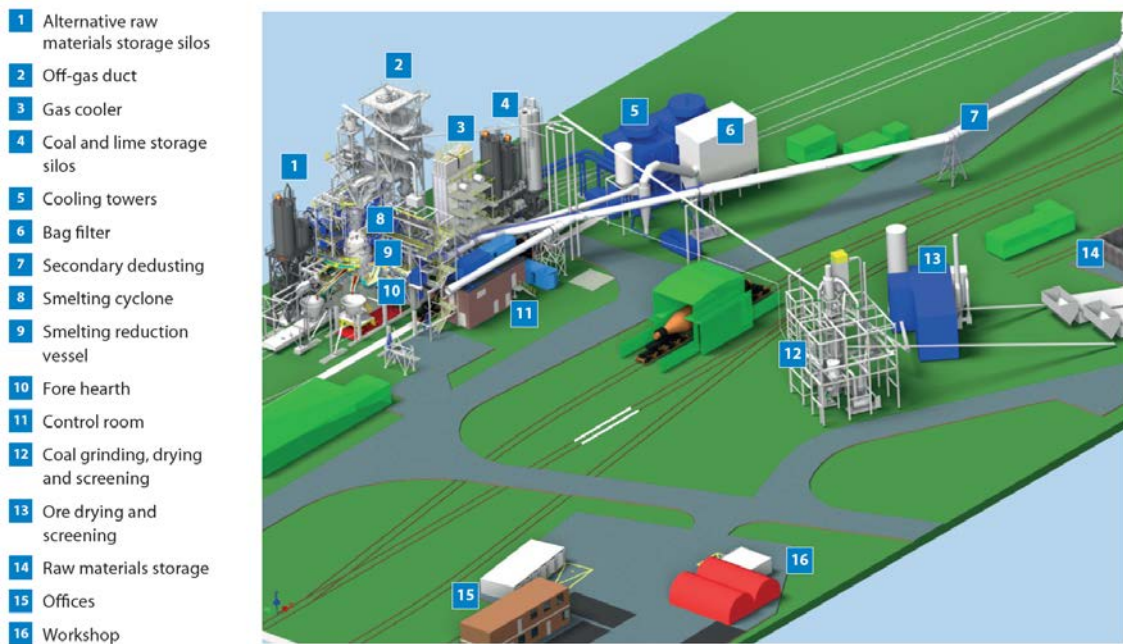
Figure 13. Layout of HIsarna pilot plant at TSIJ
