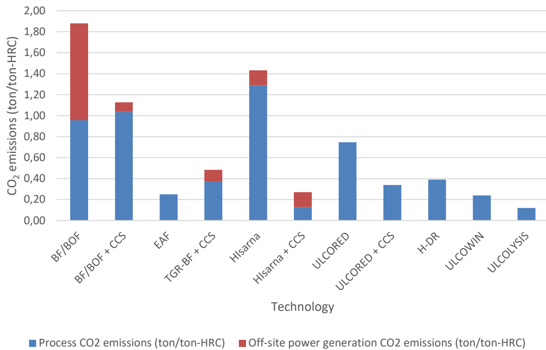
Figure 31. Comparison of CO 2 emission estimates for steelmaking technologies (excl. biomass implementation)
