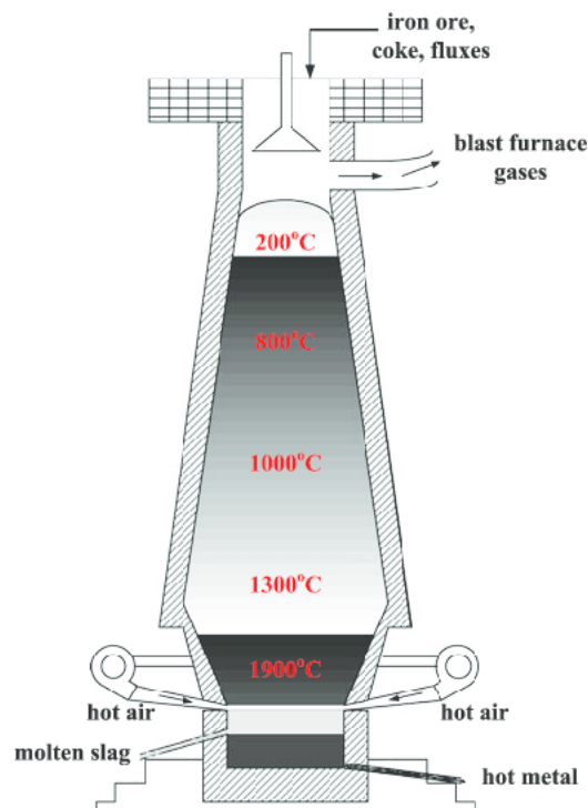
Figure 3. Schematic diagram of the blast furnace process
