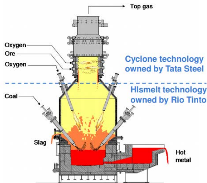
Figure 12. Simplified schematic of the HIsarna process with CCS
