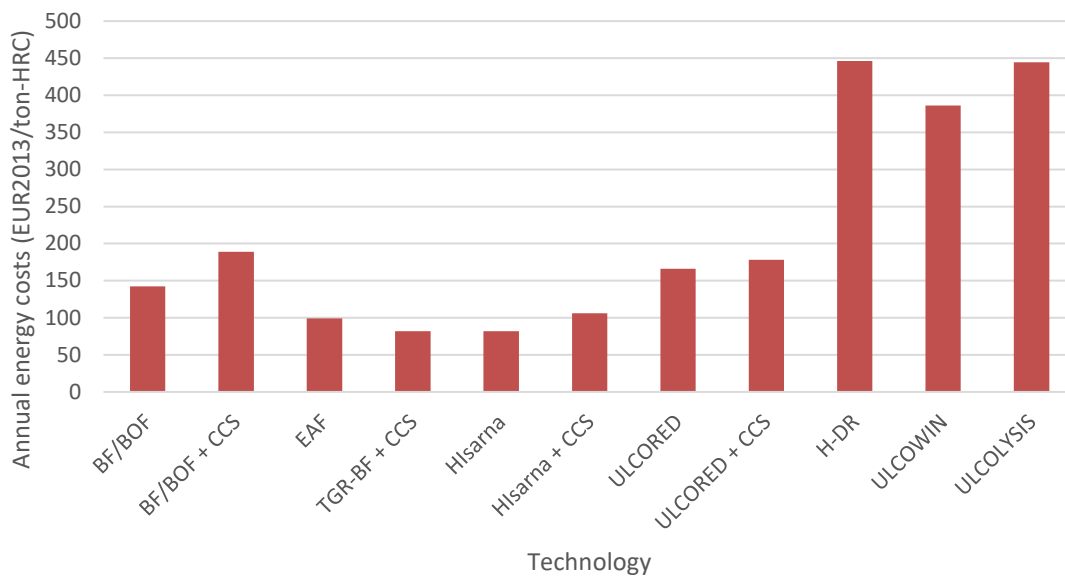
Figure 40. Annual energy costs for steelmaking options based on a 2050 high energy cost scenario in the Netherlands
