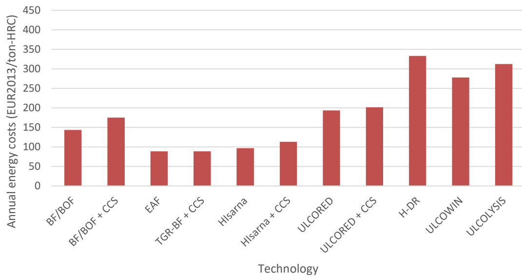
Figure 37. Annual energy costs for steelmaking options based on a 2030 low energy cost scenario in the Netherlands
