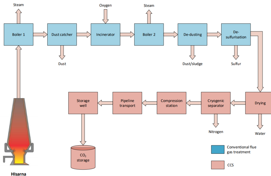
Figure 20. Systematic flowsheet of cryogenic CCS implemented to the HISarna process
