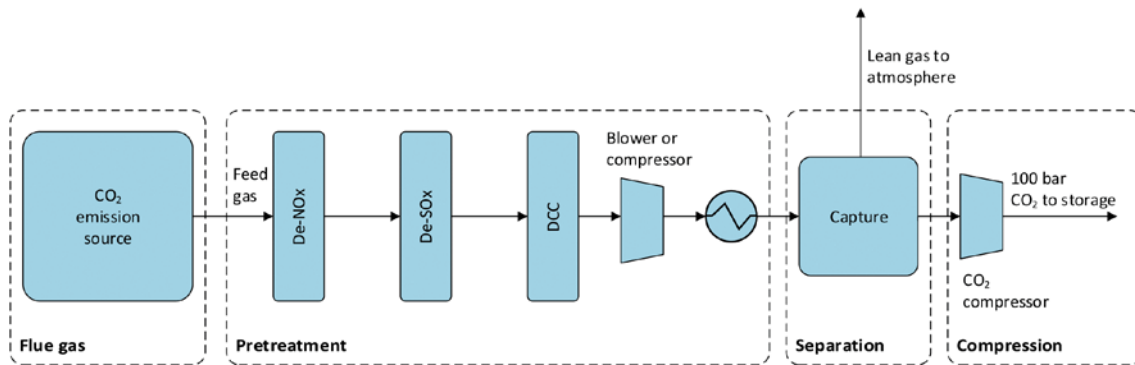
Figure 29. Scope of CO 2 capture process
