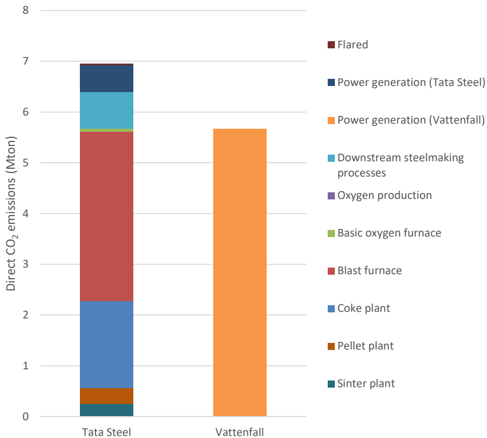
Figure 8. Calculated annual direct CO 2 emission distribution of steelmaking units and power generation plants
