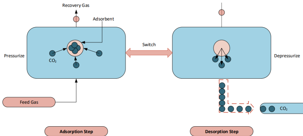
Figure 18. Basic process flow diagram of the physical adsorption-based CCS
