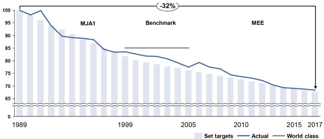
Figure 21. Energy efficiency of TSIJ overall processes relative to 1989
