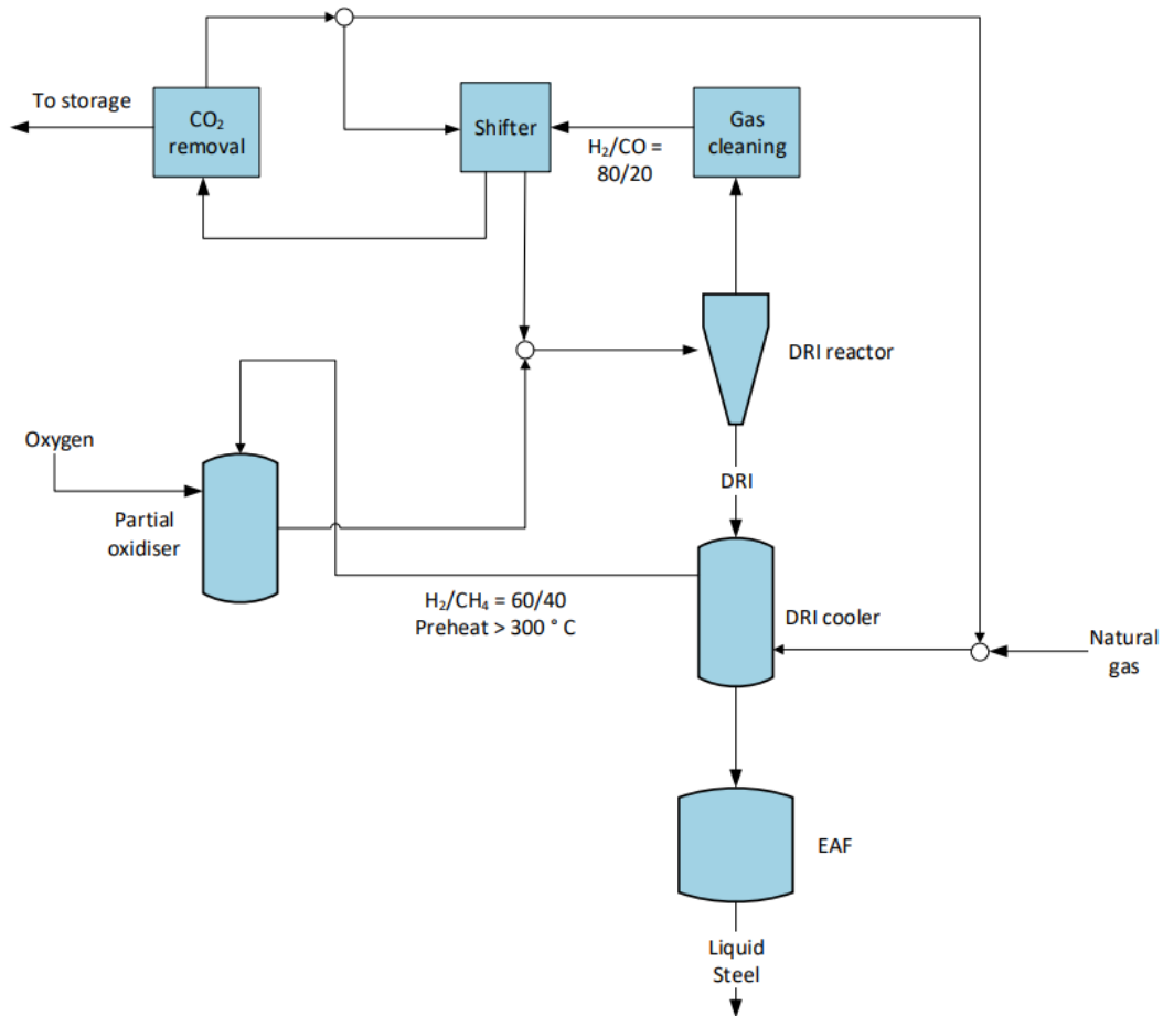
Figure 14. Basic schematic of natural gas-based ULCORED
