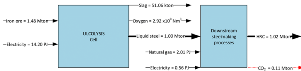
Figure 28. Flowsheet of the ULCOLYSIS steelmaking route
