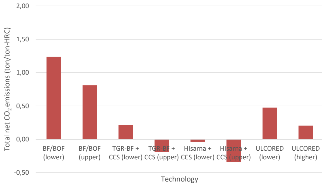
Figure 32. Comparison of CO 2 emission estimates with charcoal substitution in the most feasible steelmaking technologies
