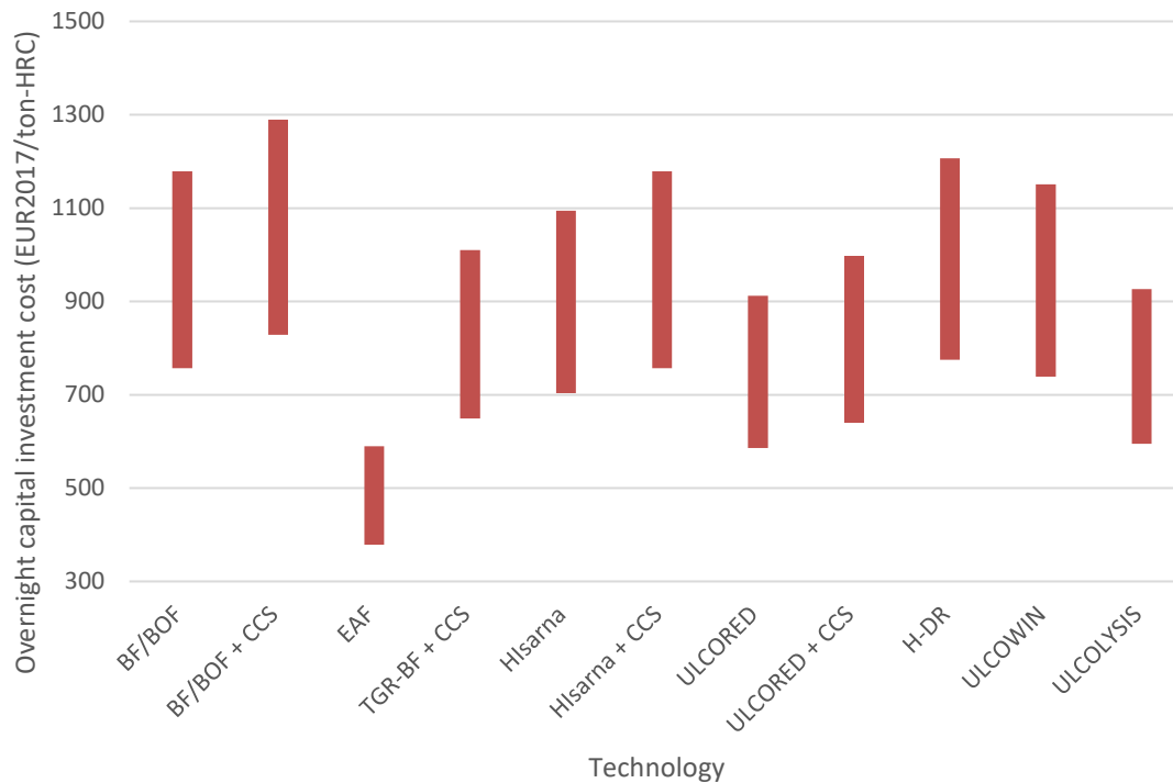
Figure 34. Overnight investment cost estimation of steelmaking decarbonisation technologies
