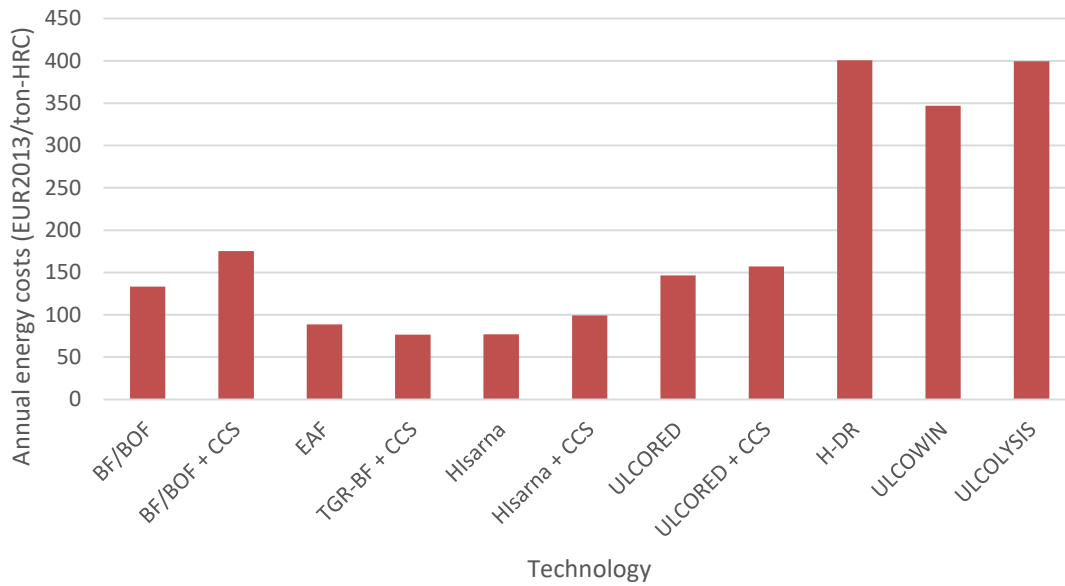
Figure 39. Annual energy costs for steelmaking options based on a 2030 high energy cost scenario in the Netherlands
