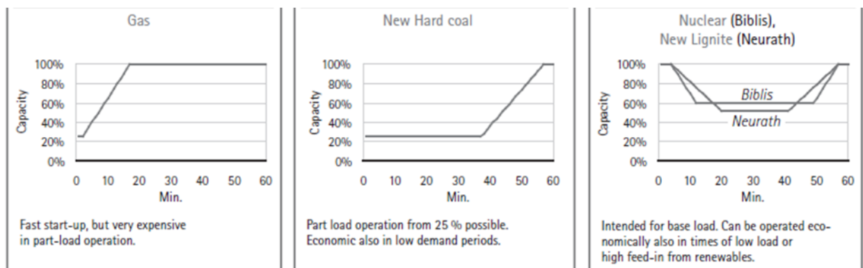
Figure 54: Power plant availability [VGB].
