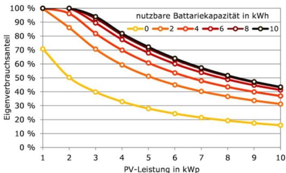
Figure 57: Percent of on-site consumption in dependence of the battery capacity and PV array power for a single-family home with an annual electricity consumption of 4,700 kWh. [Quasch]
