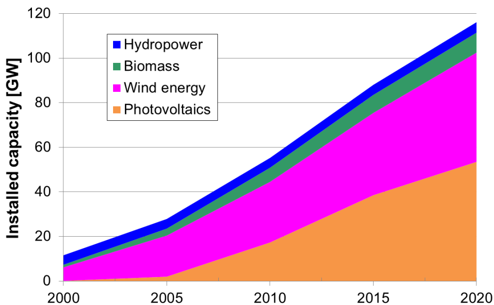
Figure 40: Scenario "2011 A" for the expansion of RE capacity, data from [IFNE].
