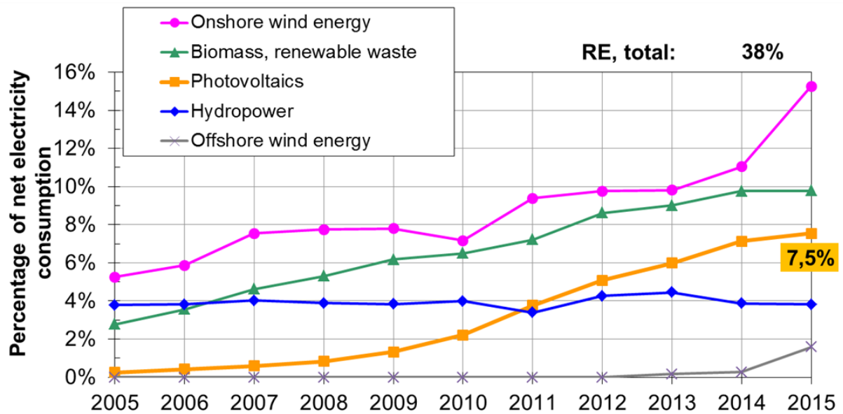
Figure 1: Percentage renewable energy in net electricity consumption (final energy) for Germany 2005-2015; data from [BMW1], [AGEB5], [AGEB6], Press Release BDEW.
