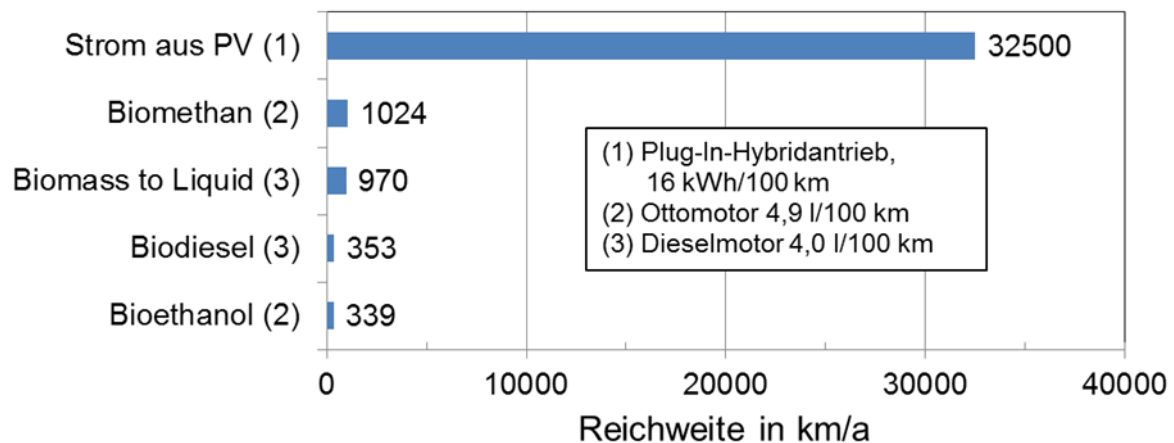
Figure 32: Vehicle range for an annual yield of 1 a = 100 m 2 of energy crops (2,3) or 40 m 2 of elevated PV modules constructed on 100 m 2 of flat open ground, Sources: Photon, April 2007 (1) and Fachagentur Nachwachsende Rohstoffe (2), (3).
