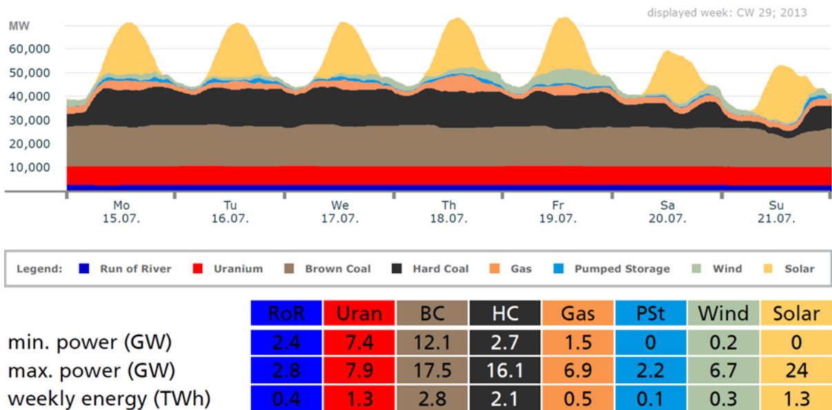
Figure 50 : Power production in 29th week of 2013, showing the current record value of 24 GW PV power generated on Sunday, July 21 with total nominal power of c. 34.5 GW (Chart: B. Burger, Fraunhofer ISE; Data: European Energy Exchange in Leipzig, EEX)
