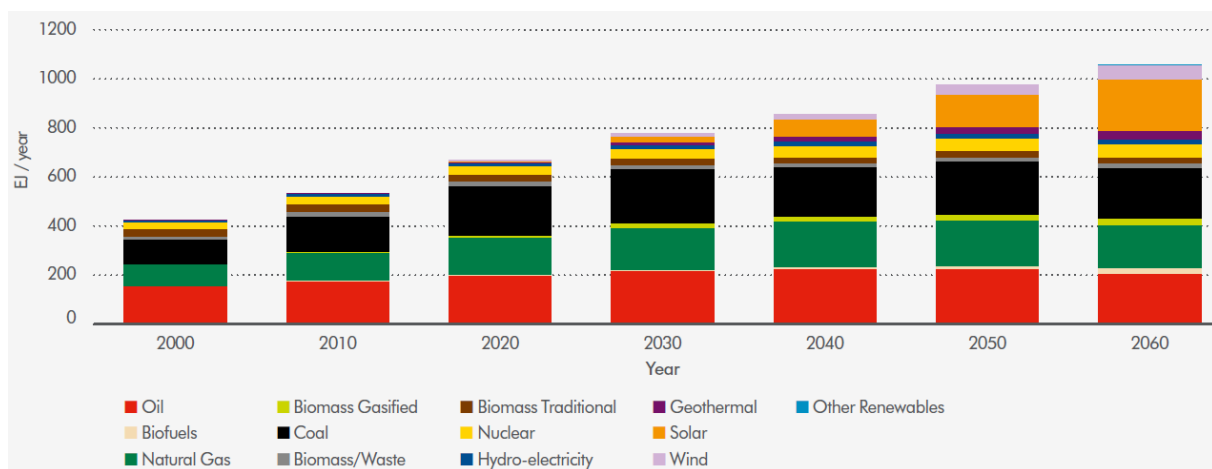
Figure 43: Primary energy consumption of various sources of power [Shell].
