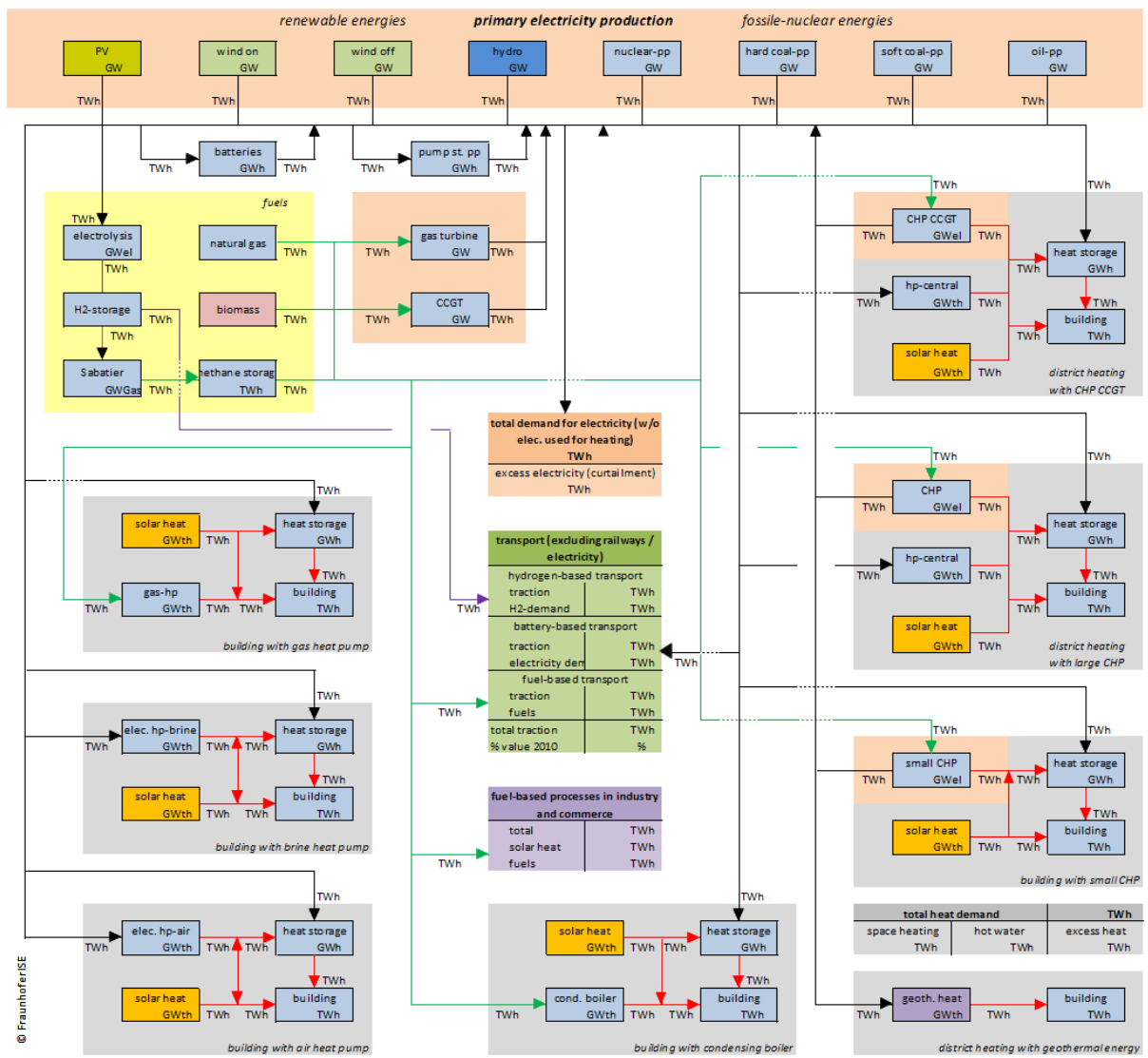
Figure 41: Scenario for Germany’s energy system, diagram of the system’s structure [ISE5].
