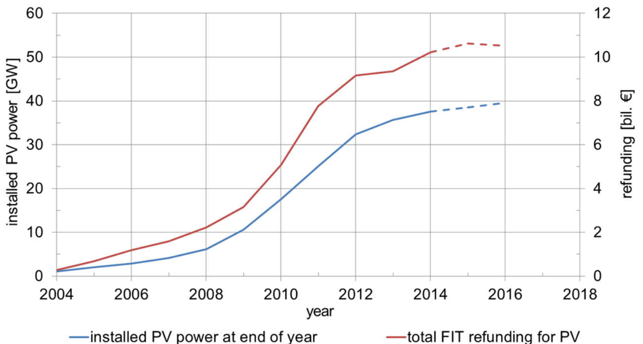
Figure 6: PV expansion and total feed-in tariff, (Data from [BMW1] and annual figures of the German grid operators; 2015 data estimated.)
