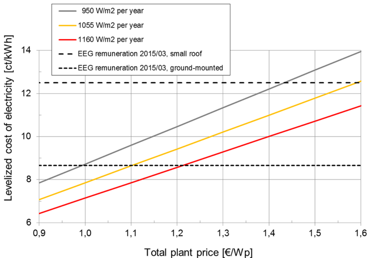
Figure 21: Rough estimate of levelized cost of electricity (LCOE) for PV power plants at different annual irradiances
