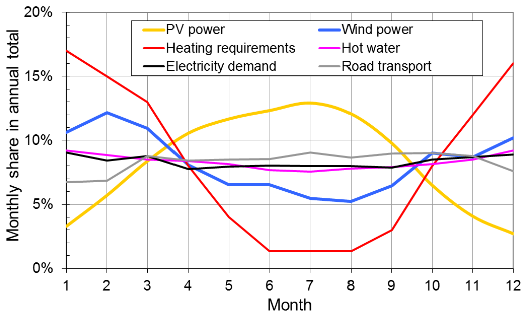
Figure 49: Rough estimate of the monthly distribution (annual total = 100 percent) of solar power calculated for Freiburg [PVGIS], wind power [DEWI], heating requirements based on the heating degree days (VDI Guideline 2067 and DIN 4713), energy requirements for domestic hot water production, electricity demand [AGEB1] and fuel requirements [MWV].
