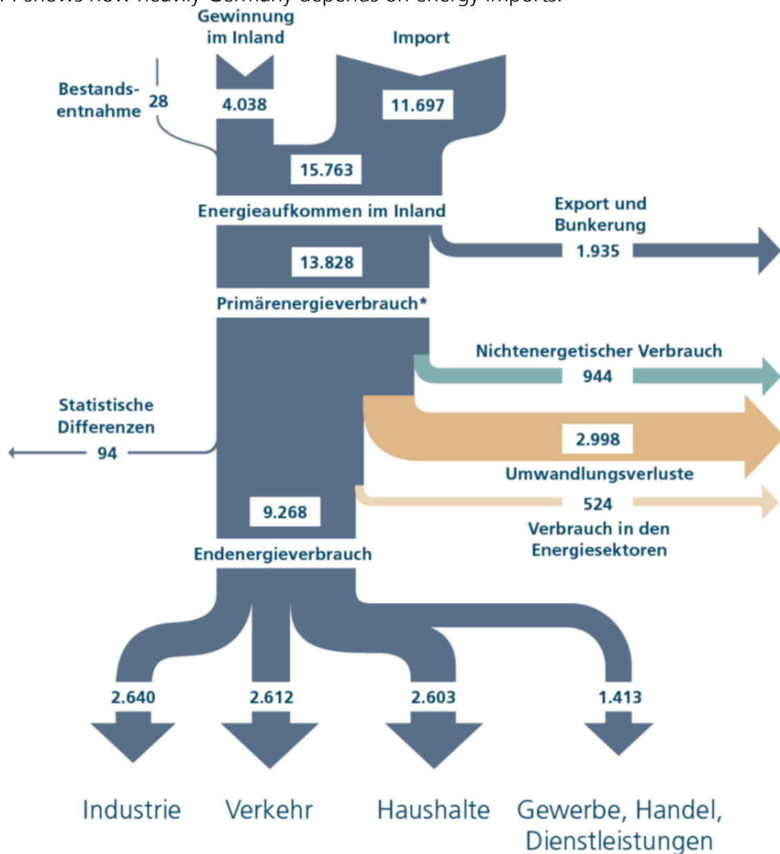
Figure 44: 2013 Energy flow diagram for the Federal Republic of Germany in petajoules (preliminary values) [AGEB2].
