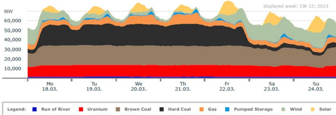
Figure 30: Example showing course of electricity trading price, conventional and renewable electricity in the 12th calendar week (March 2013)
