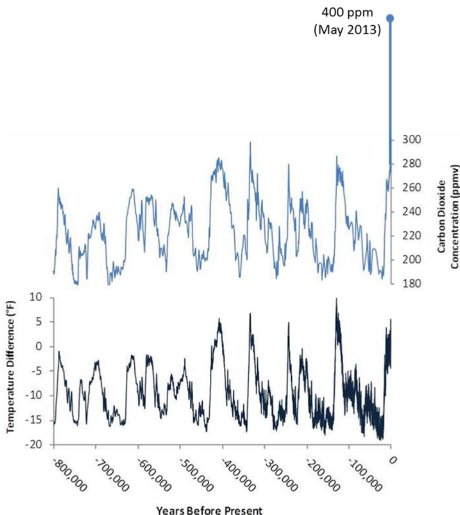
Figure 36: Estimate of the atmospheric CO 2 concentration and the temperature in Antarctica based on ice core data [EPA], CO 2 concentration for 2013 is included
