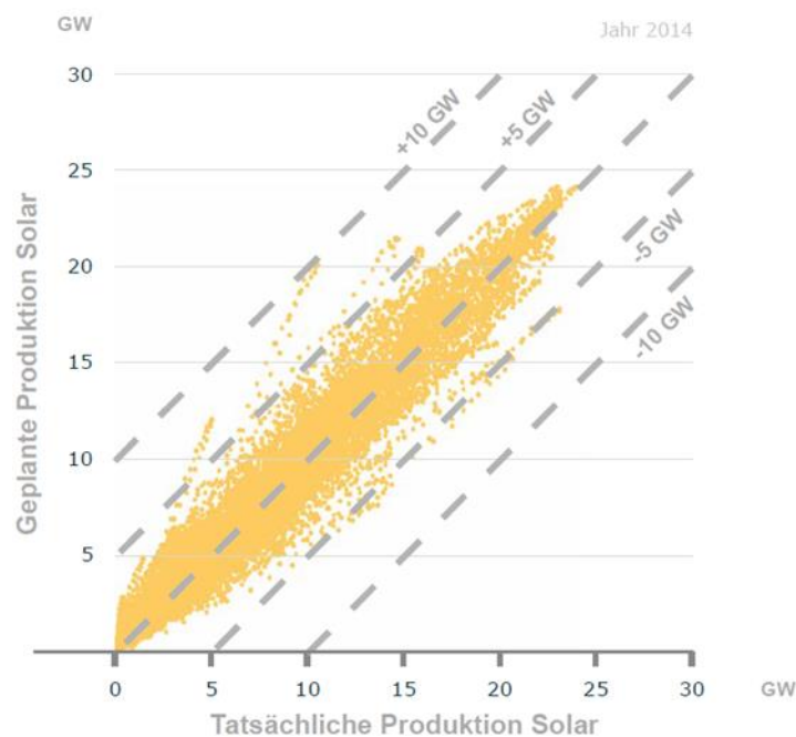
Figure 27: Actual and predicted hourly generation of power in 2014 [ISE4].
