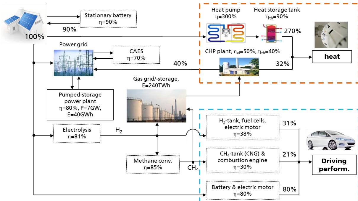
Figure 59: Possible ways of converting and storing PV power with indicative data on efficiency values.
