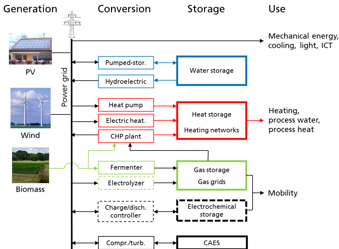
Figure 39: Simplified diagram of a renewable energy system with the most important grid-connected components for production, conversion, storage and consumption; ICT: information and communications technology; dotted lines: very low outputs/capacities currently available.
