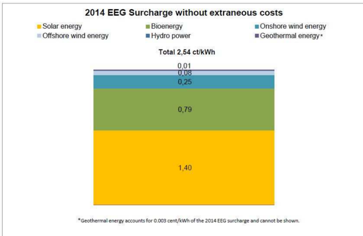
Figure 13: Breakdown of the EEG surcharge in 2014, excluding external costs [BEE1].
