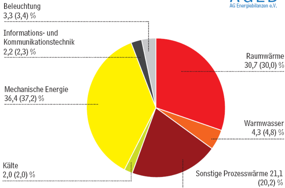
Figure 48: Different proportions of the various energy types making up Germany's final energy consumption in 2010 (data for previous year in brackets) [AGEB4].
