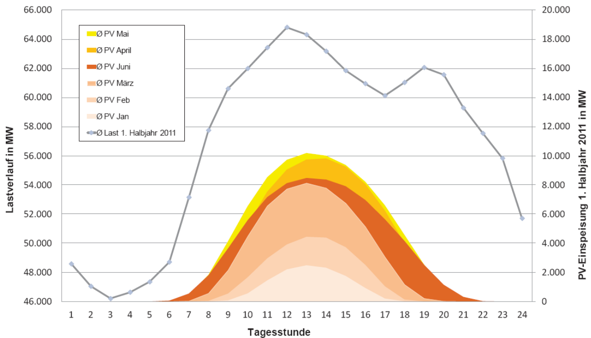
Figure 51: Average load profile and average monthly PV feed-in profiles in the first half of 2011 [IZES].
